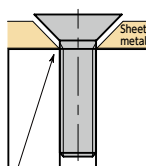
Incomplete thread part hits bottom
