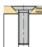
Cut seating surface prevents bottom hitting
