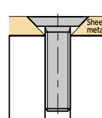
Cut seating surface prevents bottom hitting
