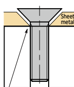
Incomplete thread part hits bottom
